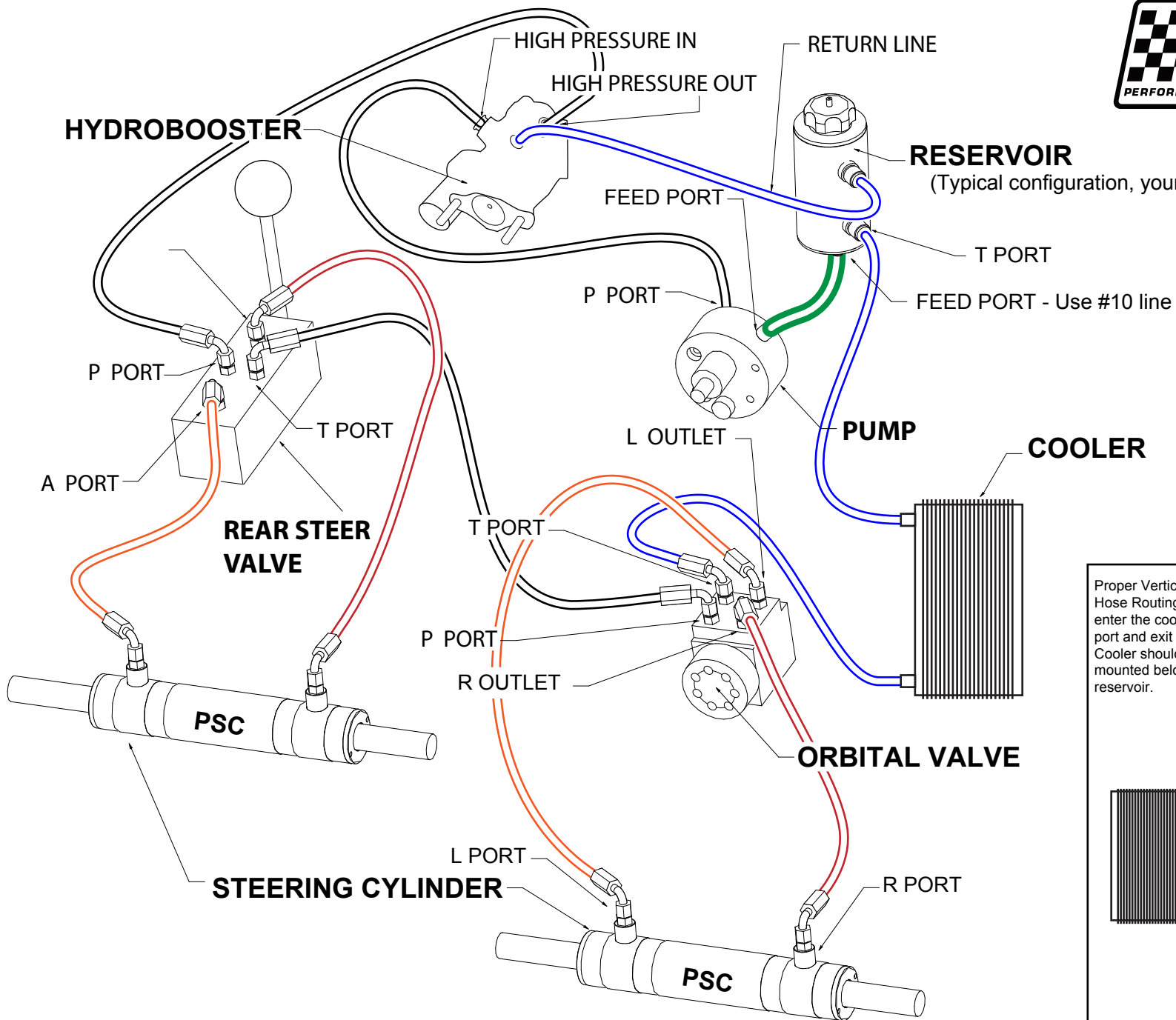
FULL HYDRAULIC HOSE ROUTING FOR FRONT AND REAR STEER APPLICATION WITH HYDROBOOST
