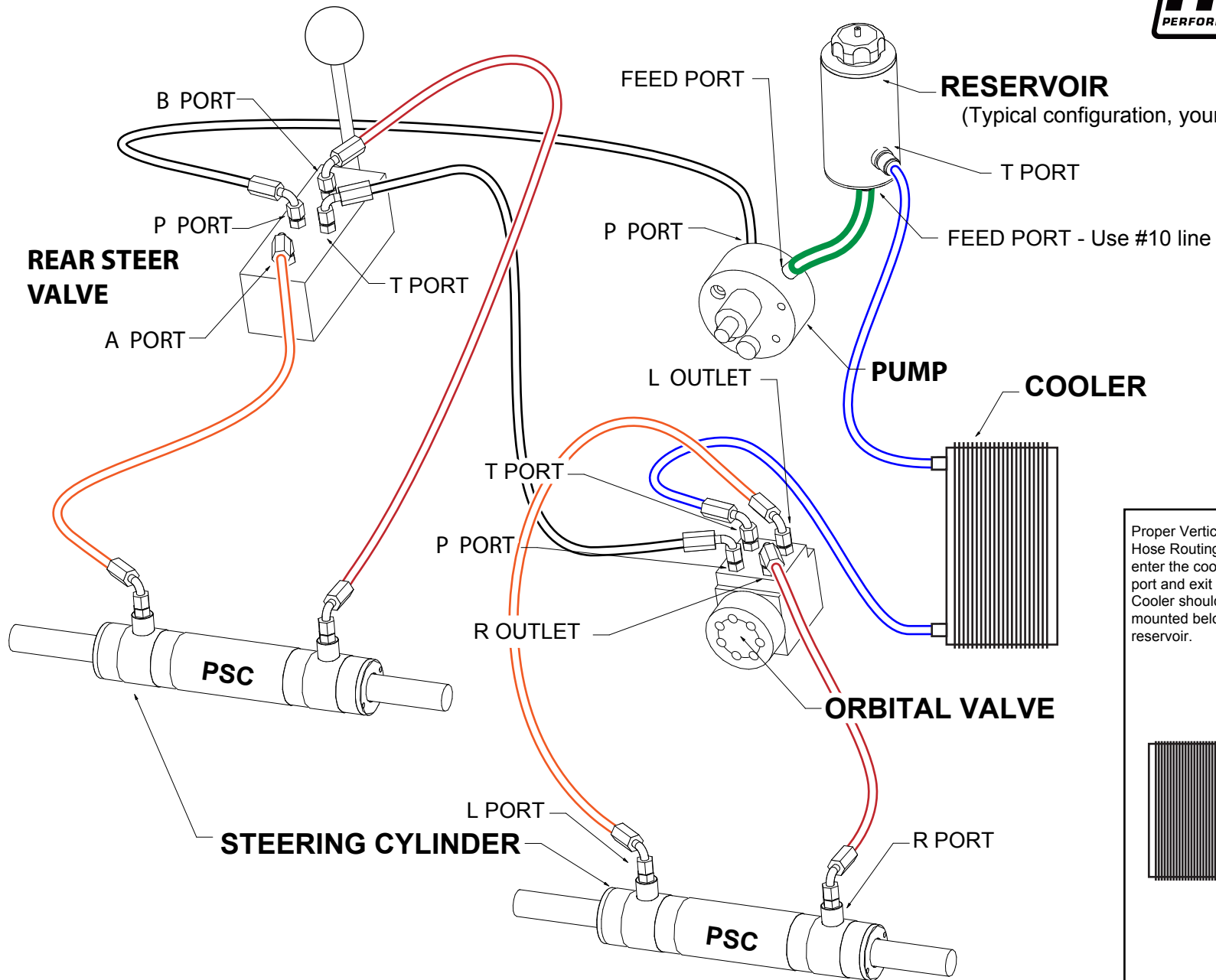
FULL HYDRAULIC HOSE ROUTING FOR FRONT AND REAR STEER APPLICATION
